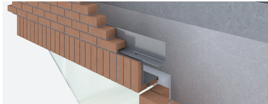
FBS installed with the FIRMA Single Leaf Lintel system
